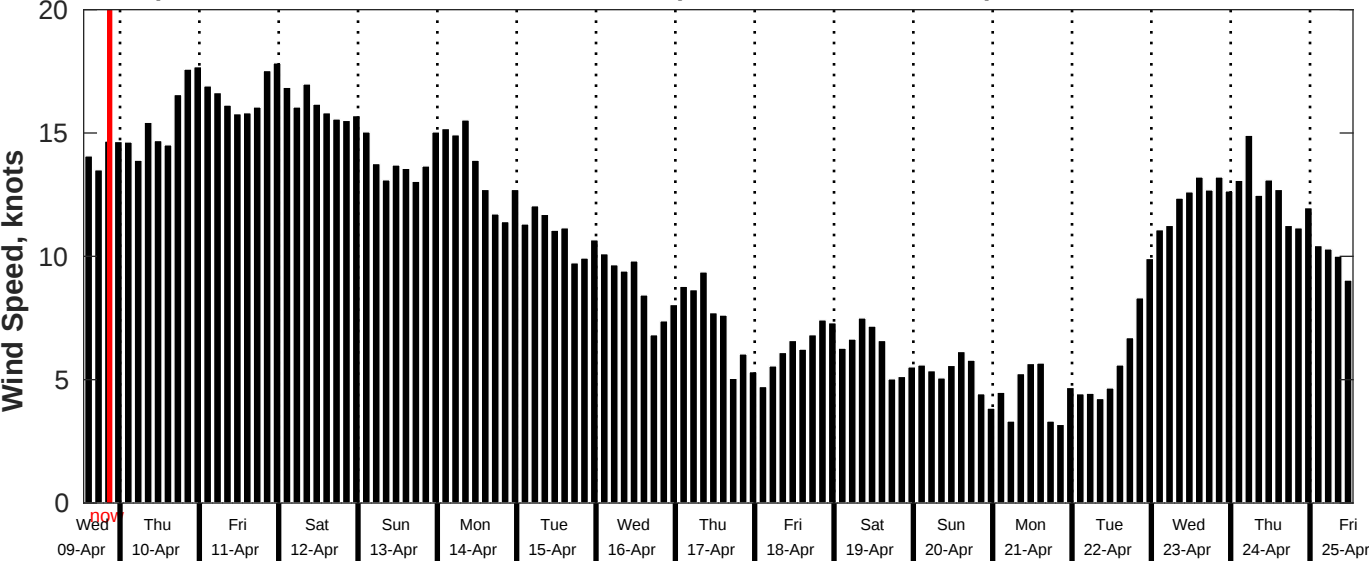
GFS Wind Speed Forecast for NDBC 51209 from 09-Apr-2025 13:00:00 to 25-Apr-2025 13:00:00
