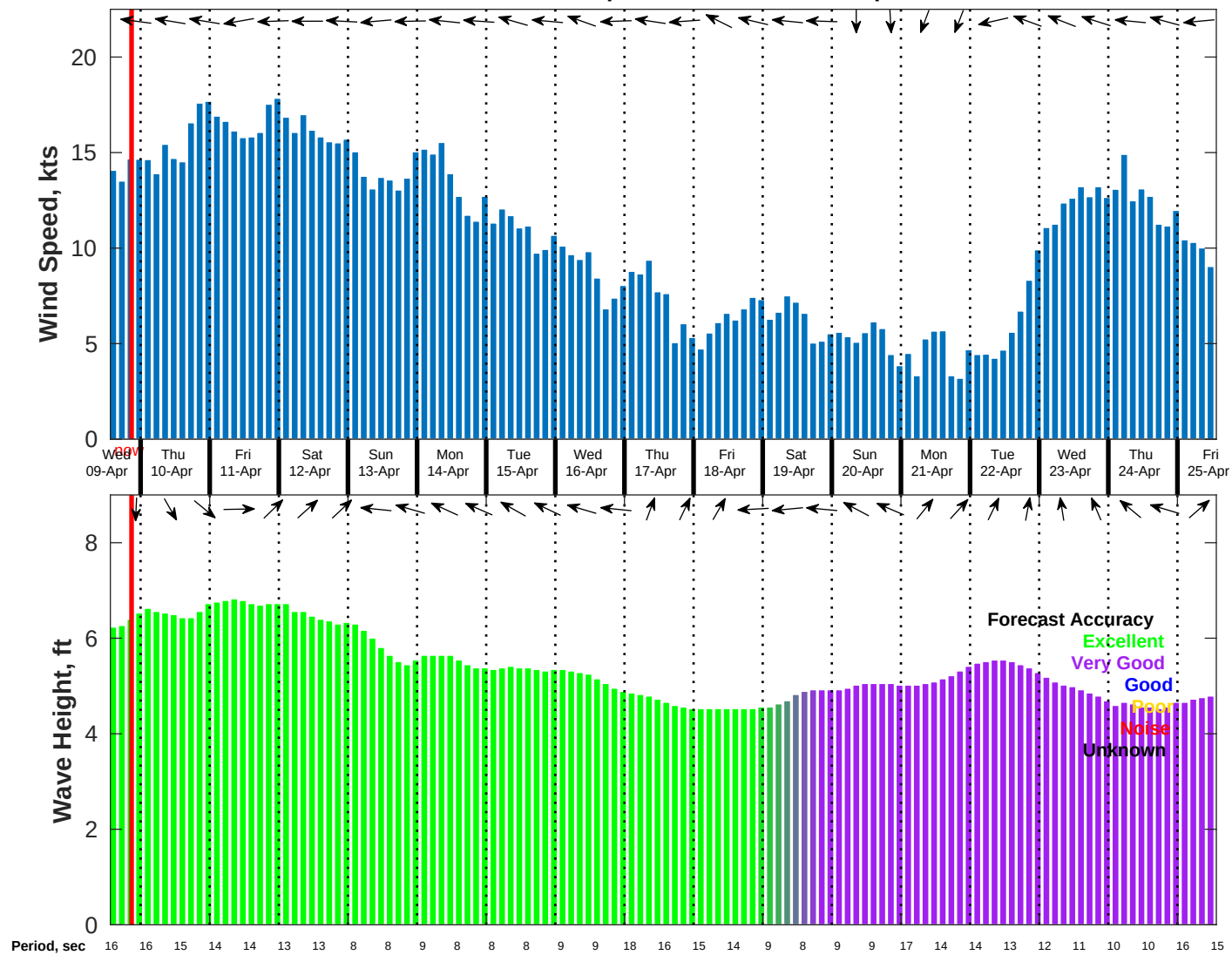
Wind & Wave Forecast for NDBC 51209 from 09-Apr-2025 13:00:00 to 25-Apr-2025 13:00:00
