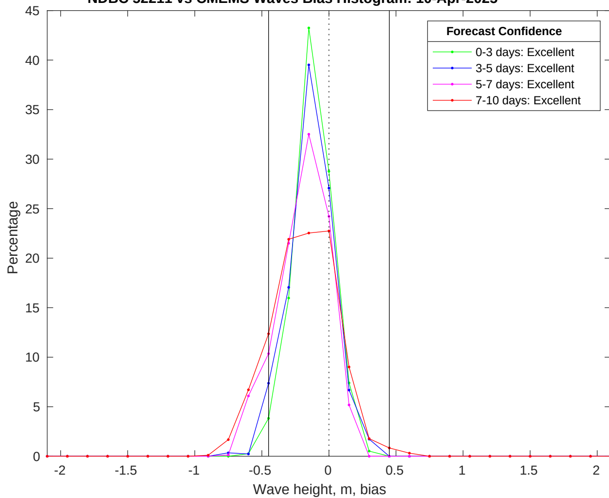
NDBC 52211 vs CMEMS Waves Bias Histogram: 10-Apr-2025
