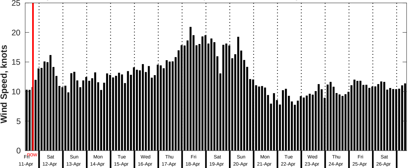
GFS Wind Speed Forecast for NDBC 52211 from 10-Apr-2025 10:00:00 to 26-Apr-2025 10:00:00
