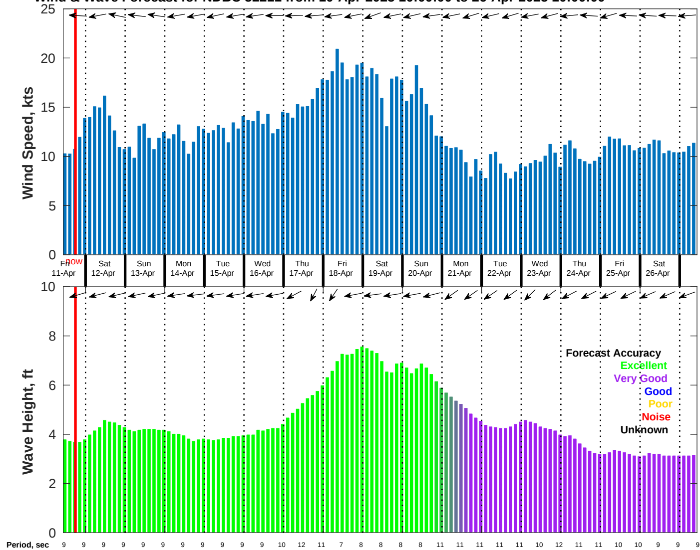
Wind & Wave Forecast for NDBC 52211 from 10-Apr-2025 10:00:00 to 26-Apr-2025 10:00:00
