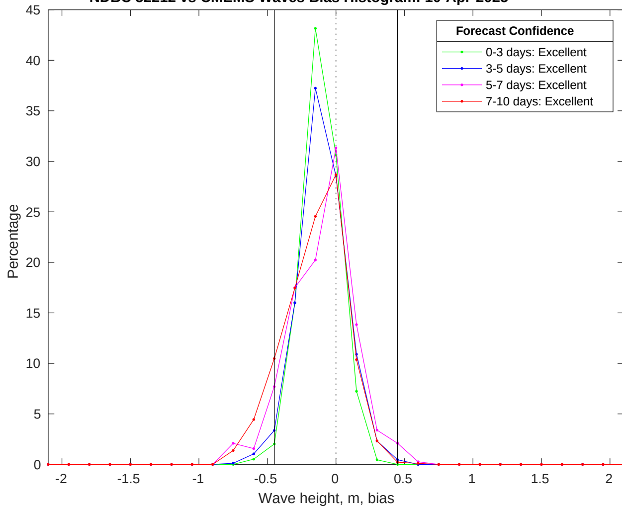
NDBC 52212 vs CMEMS Waves Bias Histogram: 10-Apr-2025
