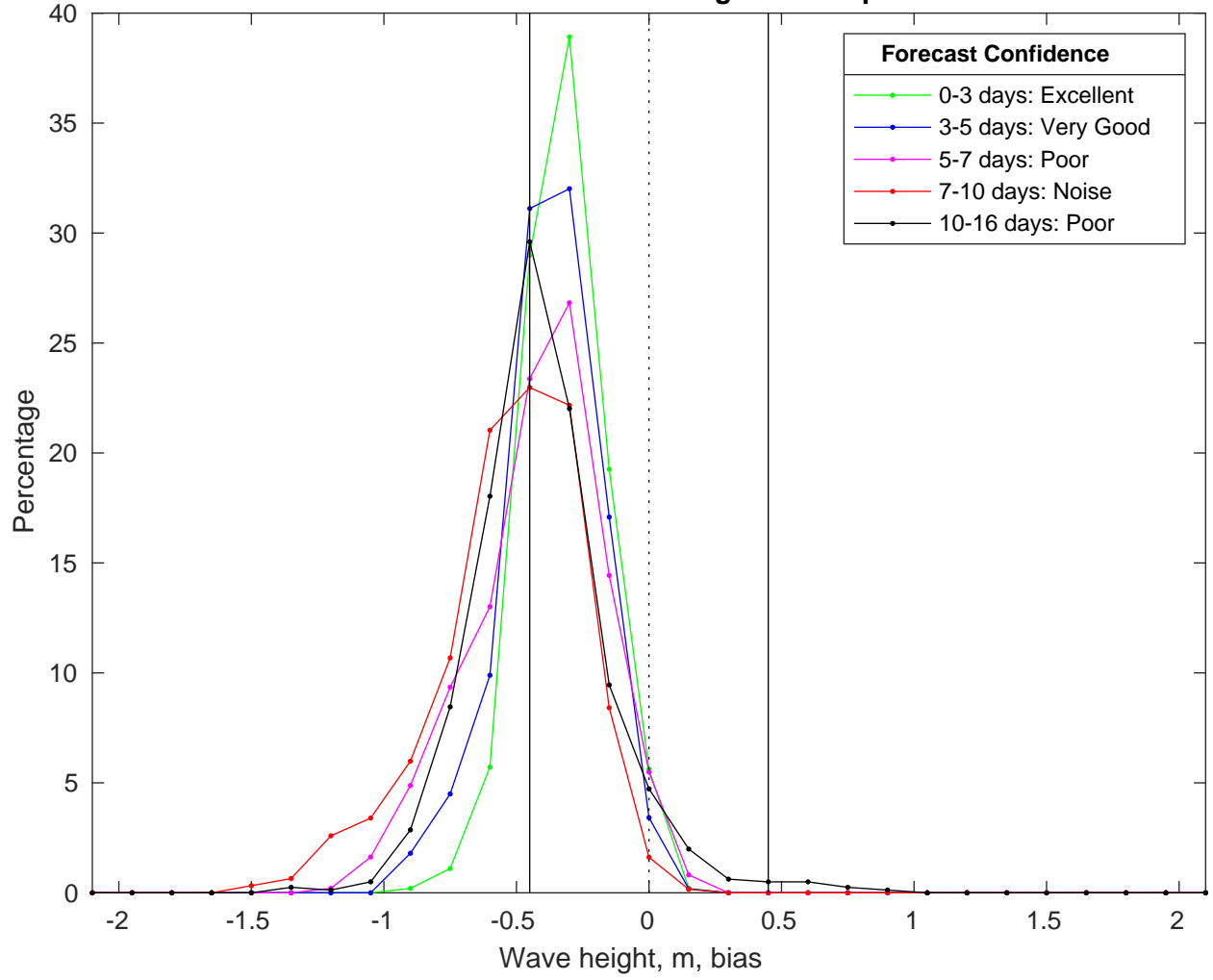
NDBC 52212 vs GFS Waves Bias Histogram: 10-Apr-2025
