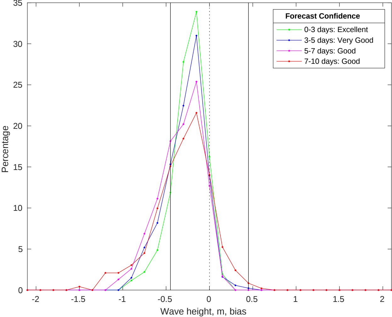
NDBC 52213 vs CMEMS Waves Bias Histogram: 10-Apr-2025
