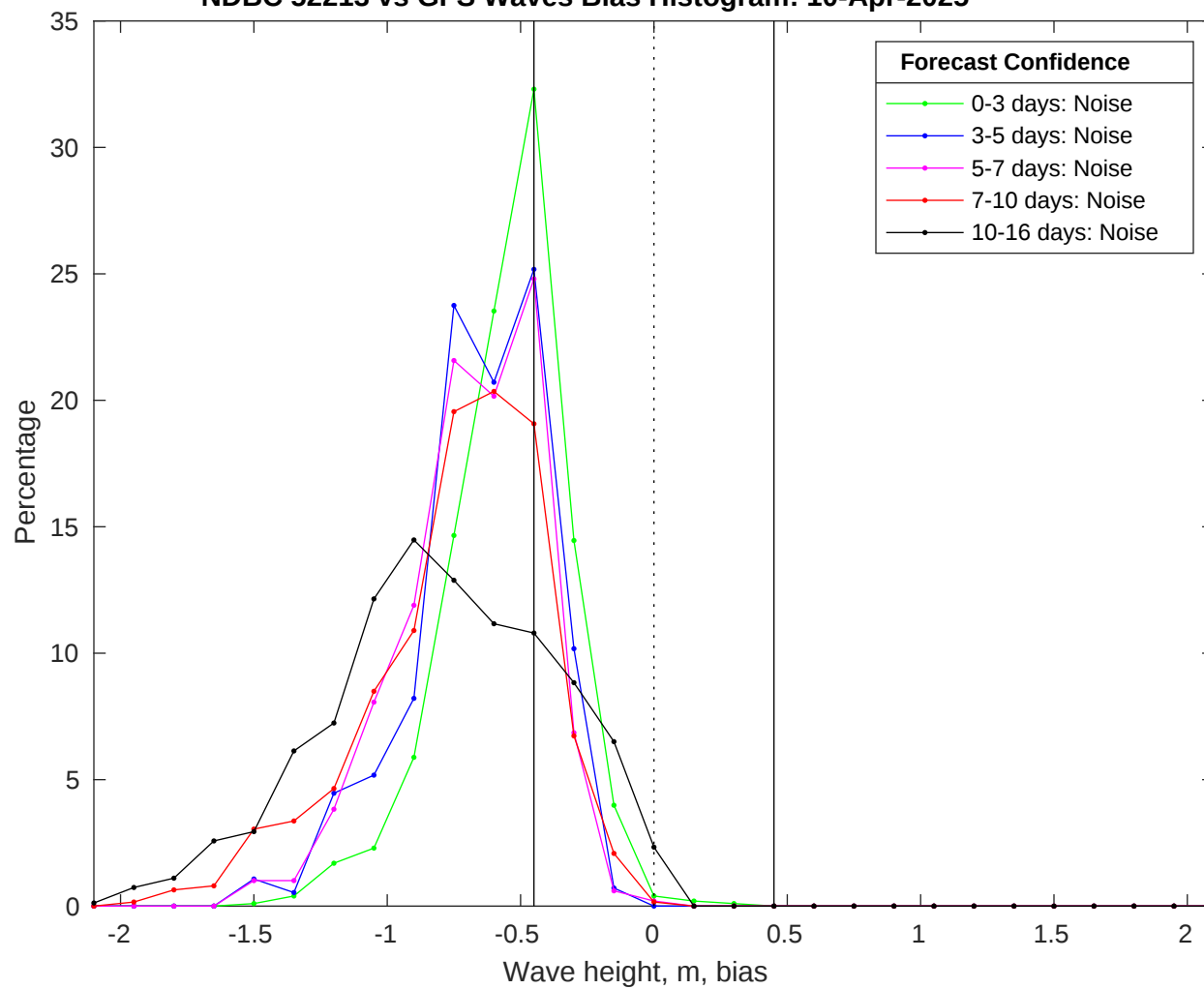
NDBC 52213 vs GFS Waves Bias Histogram: 10-Apr-2025
