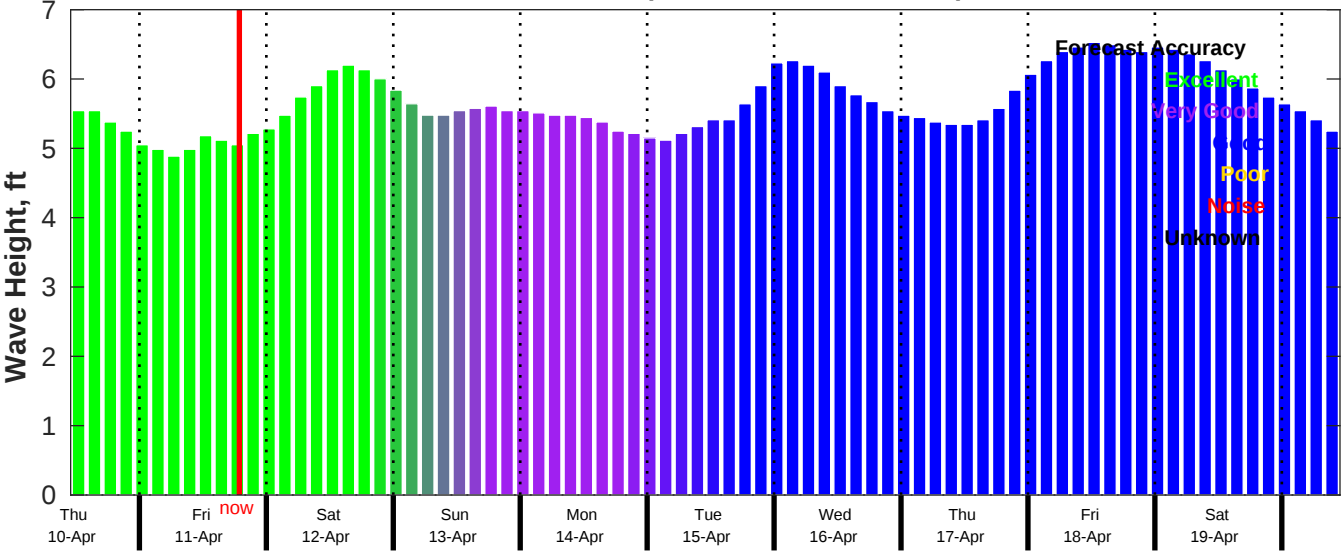
CMEMS Wave Forecast for NDBC 52213 from 09-Apr-2025 11:00:00 to 19-Apr-2025 11:00:00
