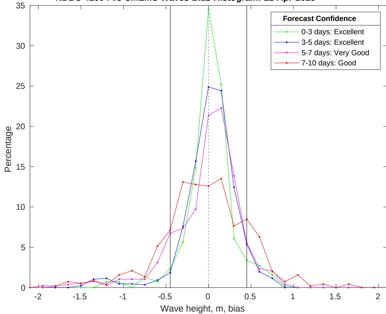
NDBC 41004 vs CMEMS Waves Bias Histogram: 11-Apr-2025
