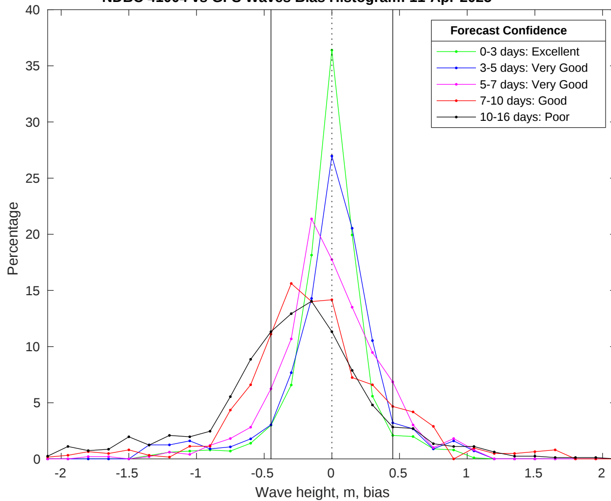
NDBC 41004 vs GFS Waves Bias Histogram: 11-Apr-2025
