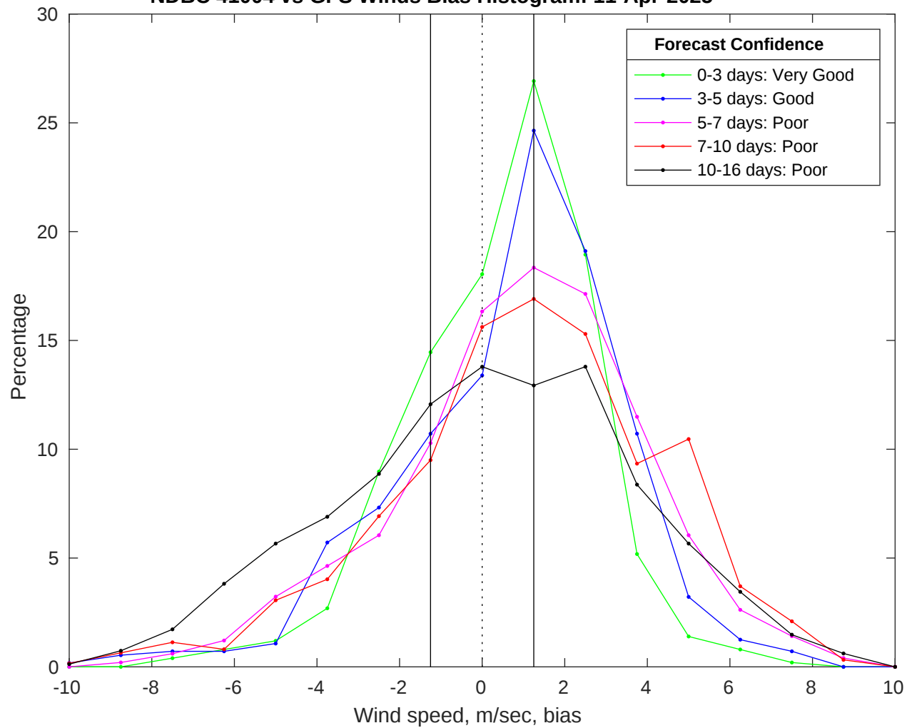
NDBC 41004 vs GFS Winds Bias Histogram: 11-Apr-2025
