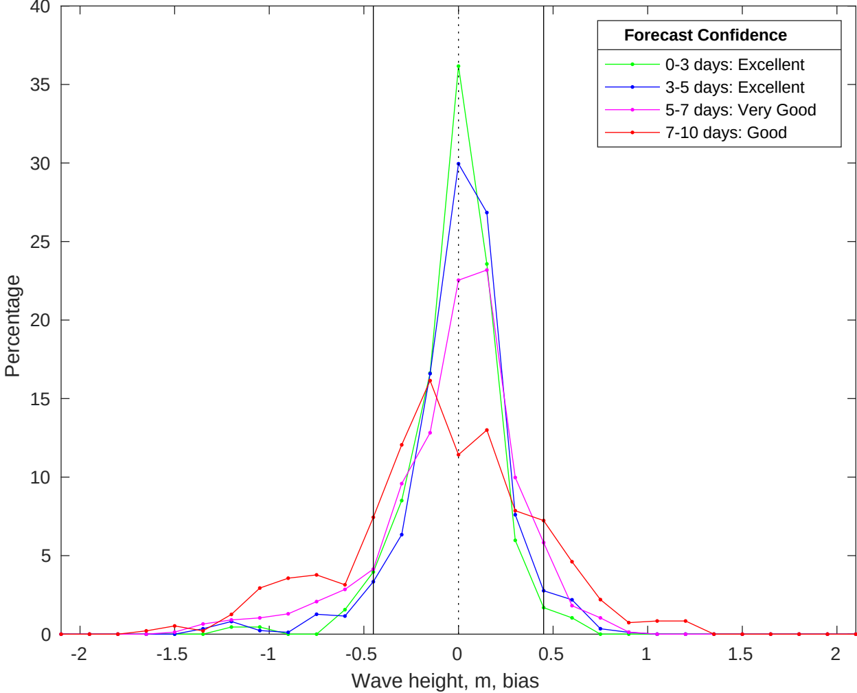
NDBC 41013 vs CMEMS Waves Bias Histogram: 11-Apr-2025
