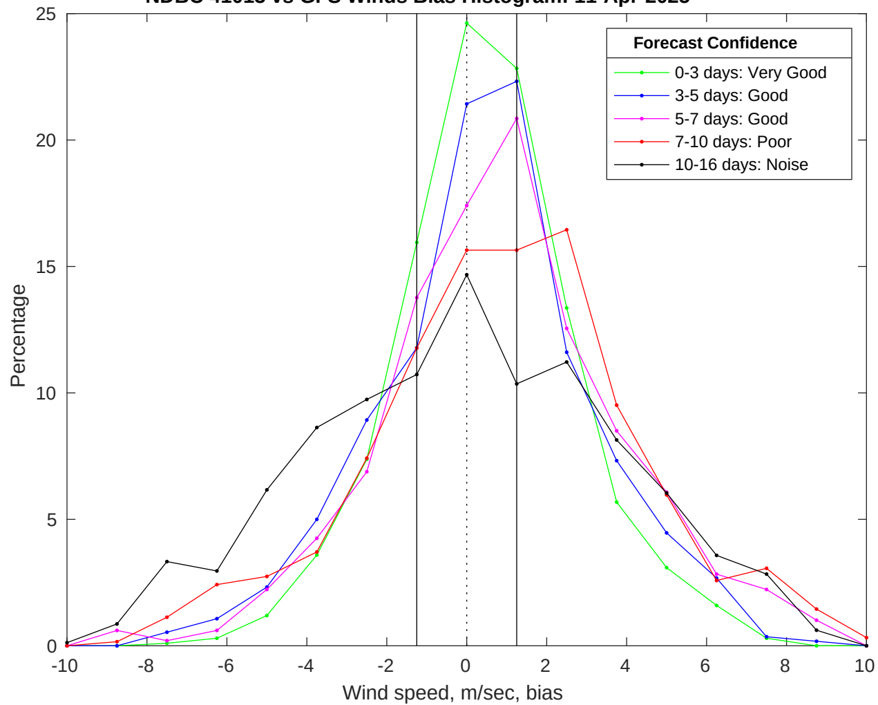
NDBC 41013 vs GFS Winds Bias Histogram: 11-Apr-2025
