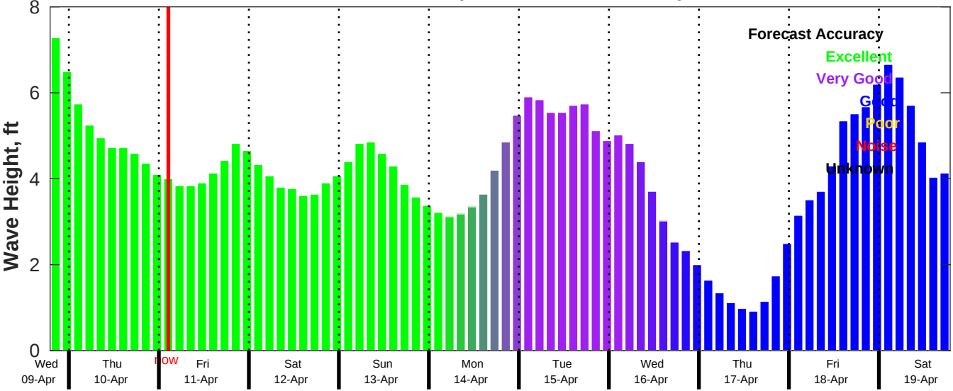
CMEMS Wave Forecast for NDBC 41013 from 09-Apr-2025 19:00:00 to 19-Apr-2025 19:00:00
