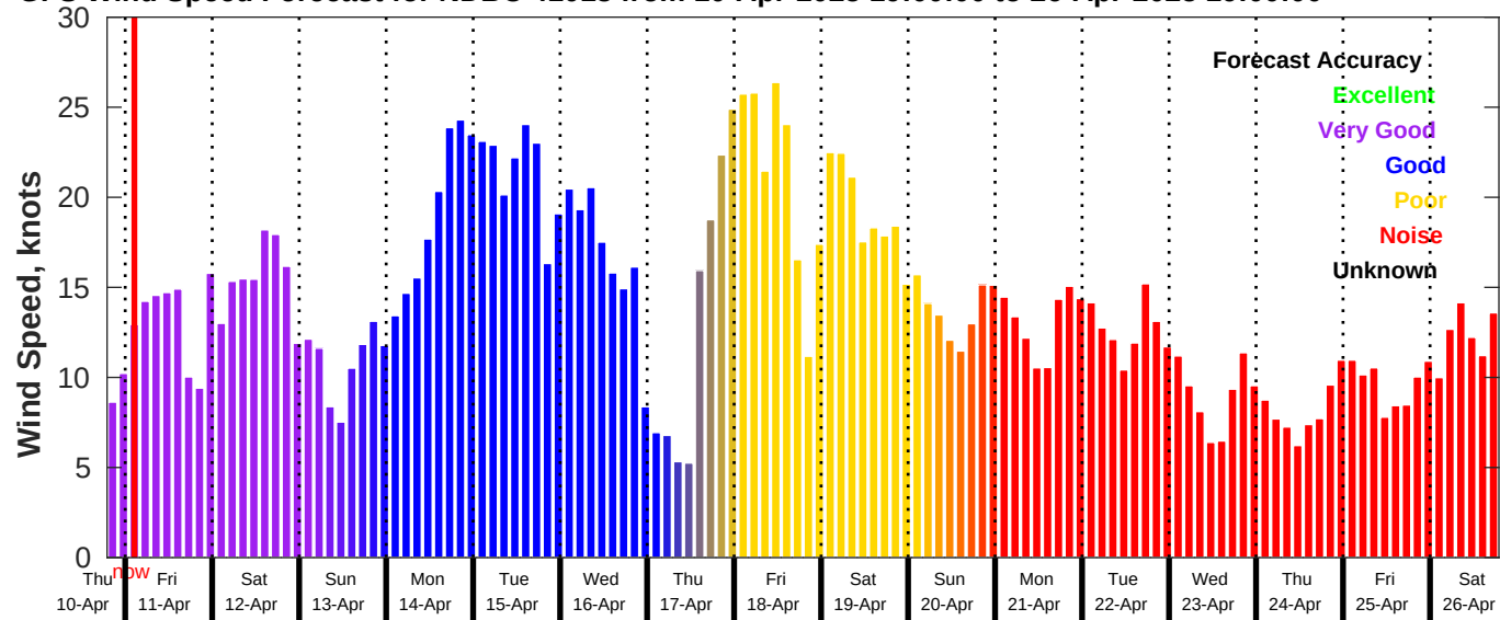
GFS Wind Speed Forecast for NDBC 41013 from 10-Apr-2025 19:00:00 to 26-Apr-2025 19:00:00
