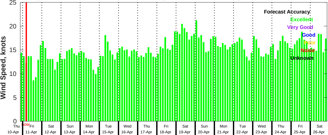
GFS Wind Speed Forecast for NDBC 41040 from 10-Apr-2025 21:00:00 to 26-Apr-2025 21:00:00
