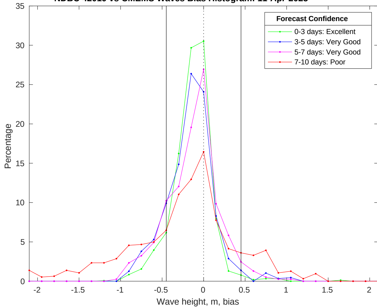
NDBC 42019 vs CMEMS Waves Bias Histogram: 11-Apr-2025
