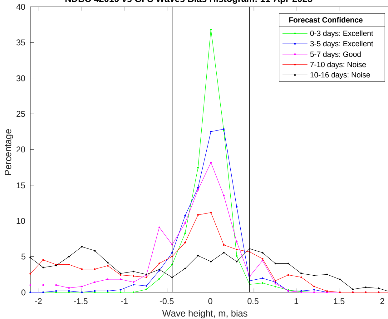
NDBC 42019 vs GFS Waves Bias Histogram: 11-Apr-2025
