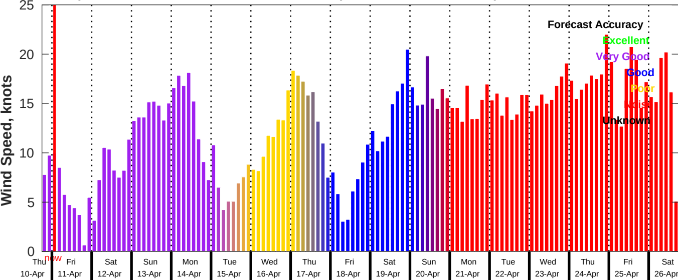
GFS Wind Speed Forecast for NDBC 42019 from 10-Apr-2025 18:00:00 to 26-Apr-2025 18:00:00
