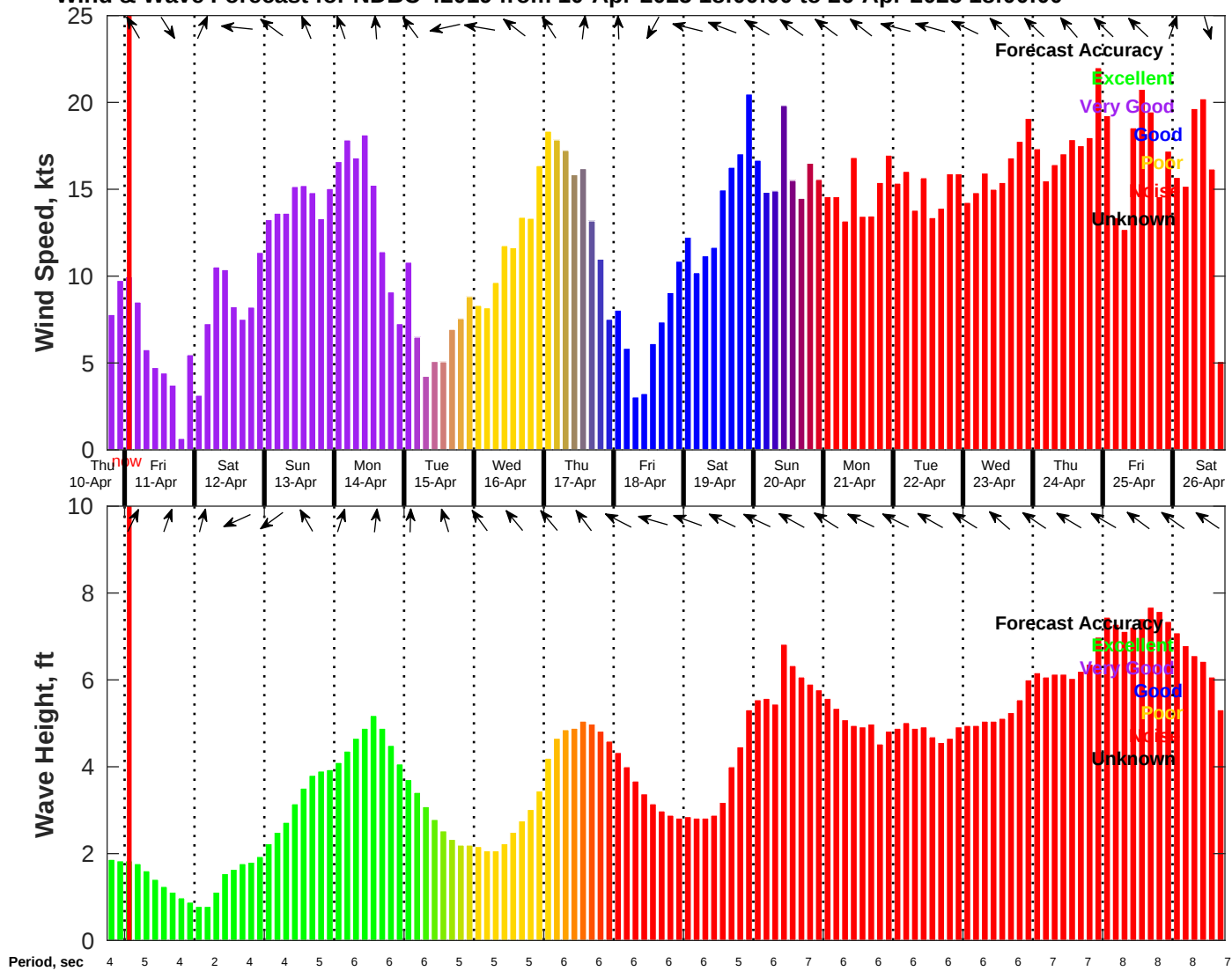
Wind & Wave Forecast for NDBC 42019 from 10-Apr-2025 18:00:00 to 26-Apr-2025 18:00:00
