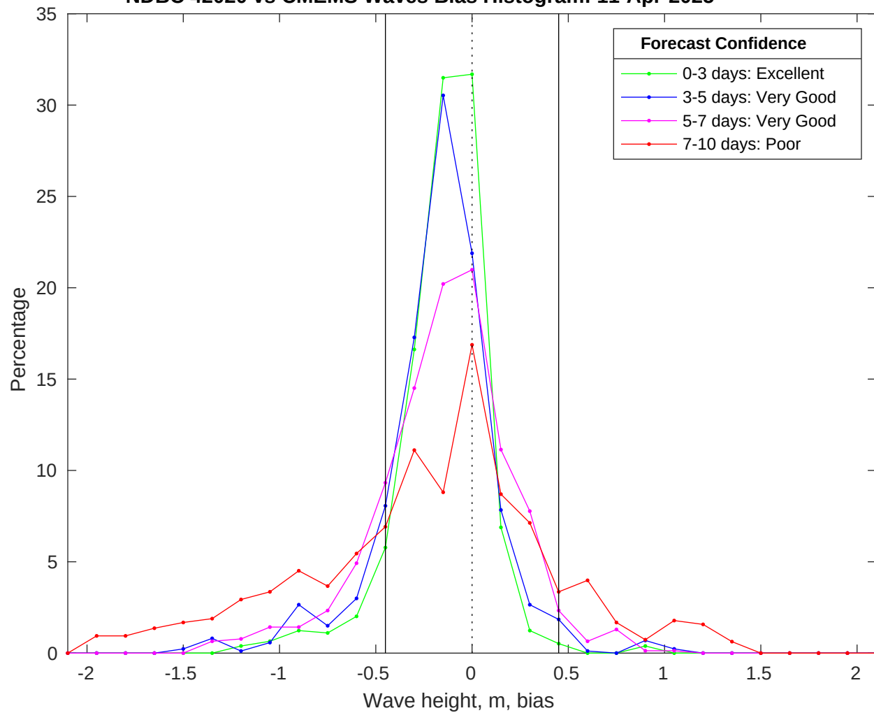
NDBC 42020 vs CMEMS Waves Bias Histogram: 11-Apr-2025
