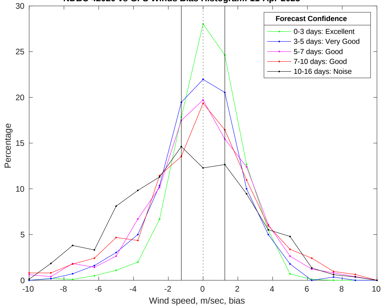
NDBC 42020 vs GFS Winds Bias Histogram: 11-Apr-2025
