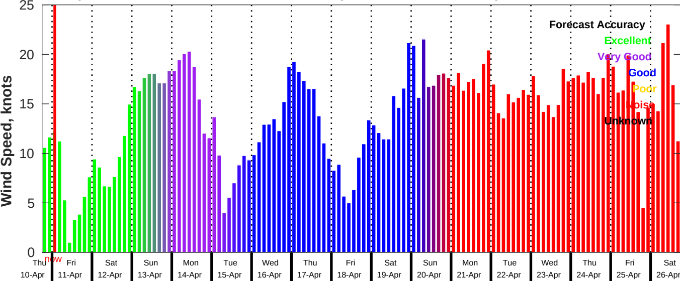
GFS Wind Speed Forecast for NDBC 42020 from 10-Apr-2025 18:00:00 to 26-Apr-2025 18:00:00
