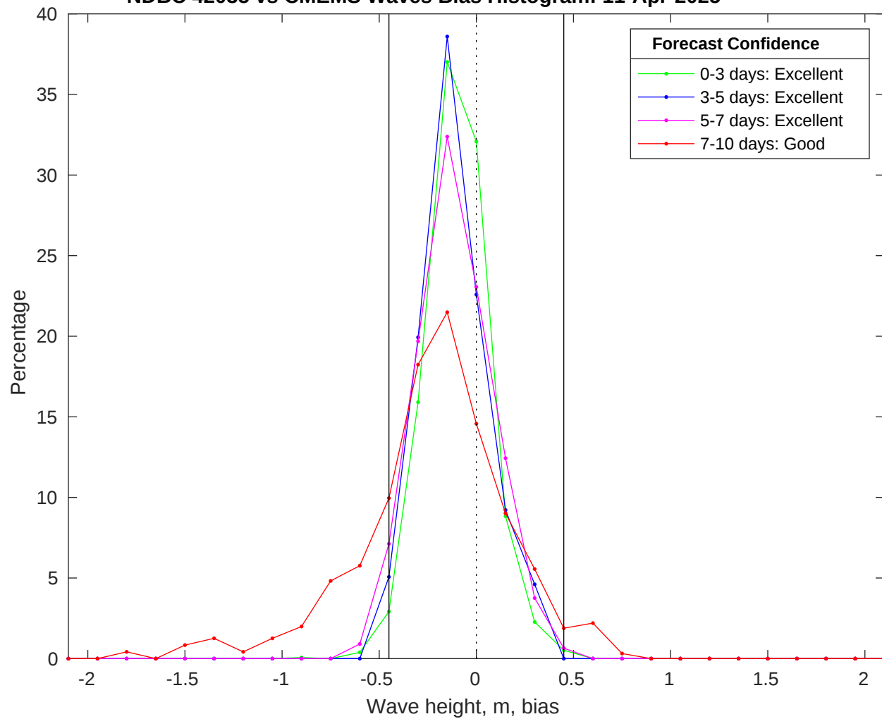
NDBC 42035 vs CMEMS Waves Bias Histogram: 11-Apr-2025
