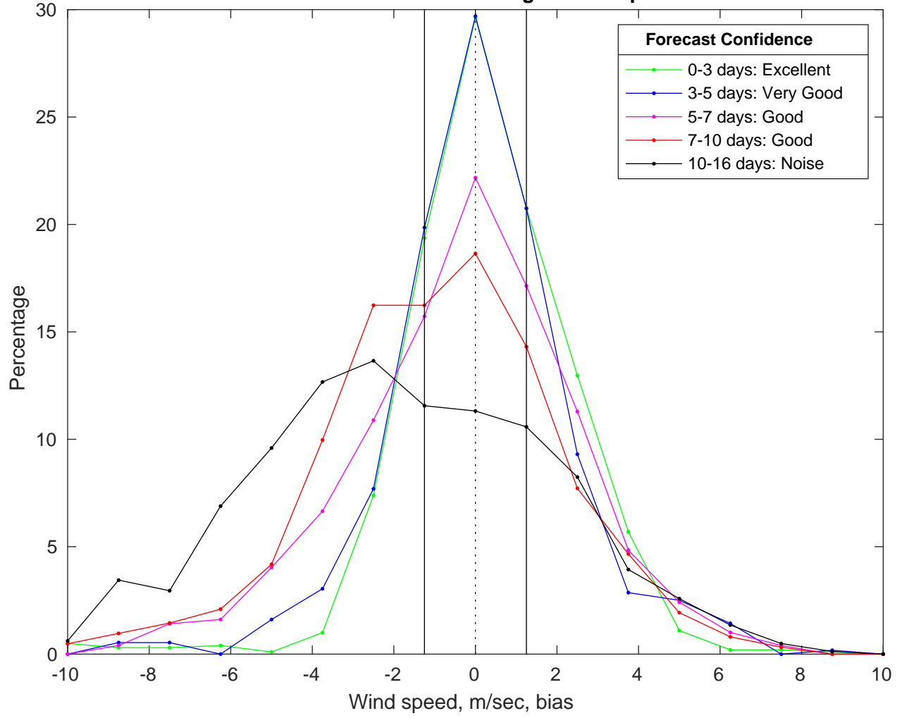
NDBC 42035 vs GFS Winds Bias Histogram: 11-Apr-2025
