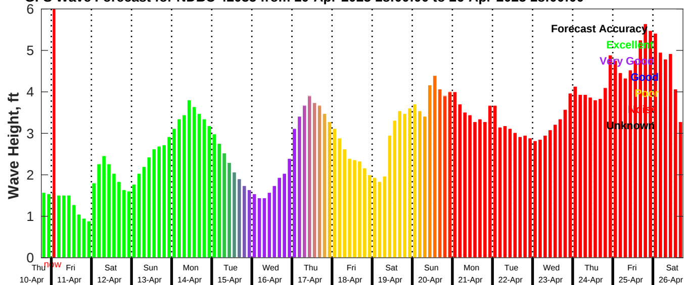
GFS Wave Forecast for NDBC 42035 from 10-Apr-2025 18:00:00 to 26-Apr-2025 18:00:00
