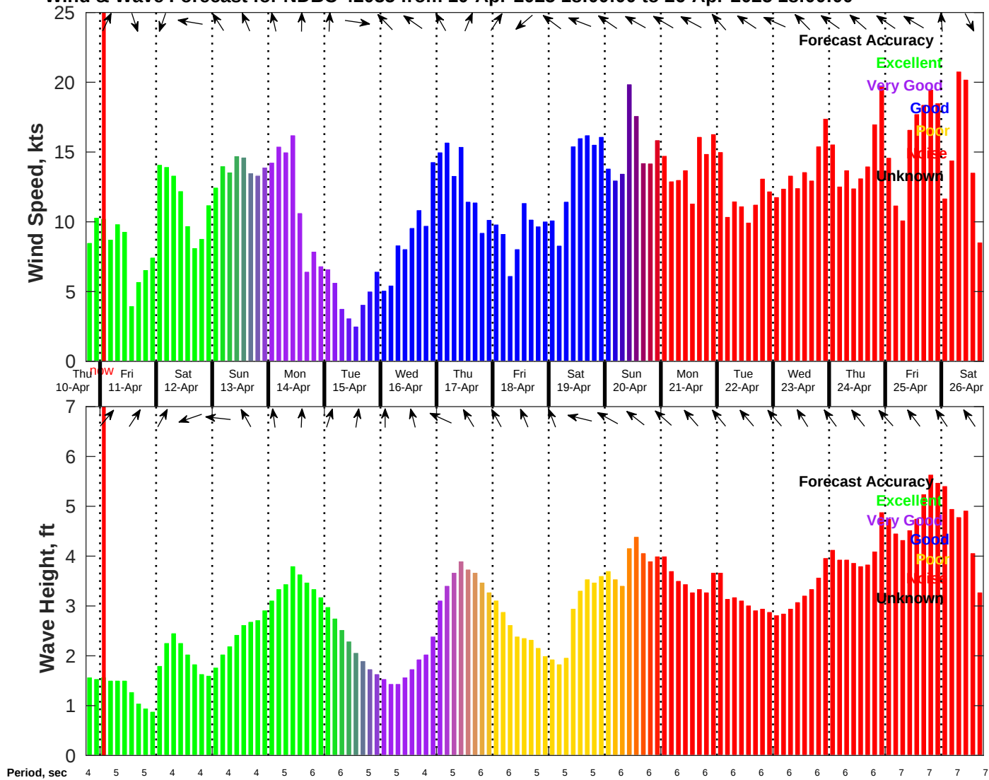
Wind & Wave Forecast for NDBC 42035 from 10-Apr-2025 18:00:00 to 26-Apr-2025 18:00:00
