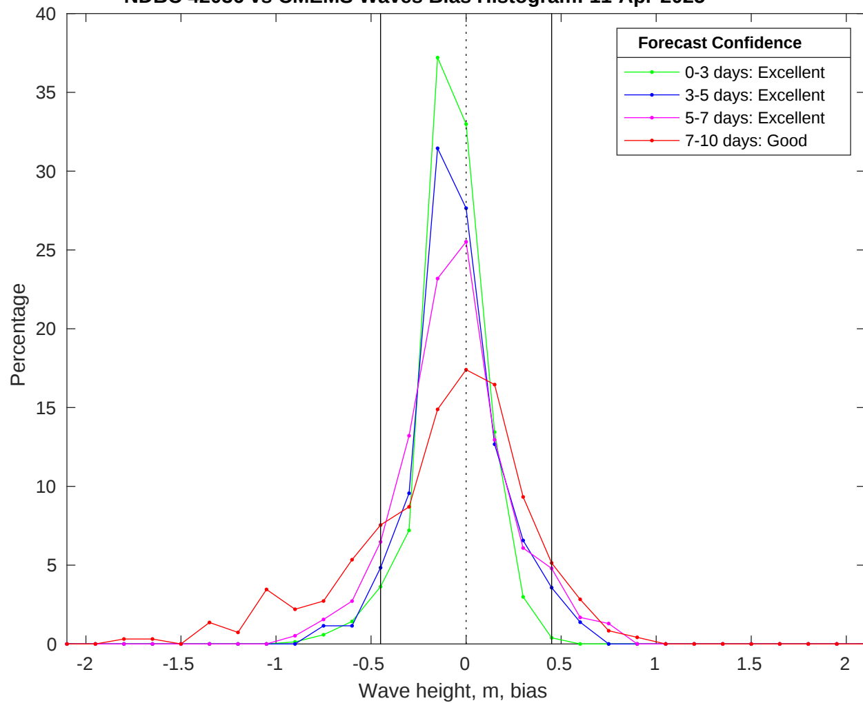
NDBC 42036 vs CMEMS Waves Bias Histogram: 11-Apr-2025
