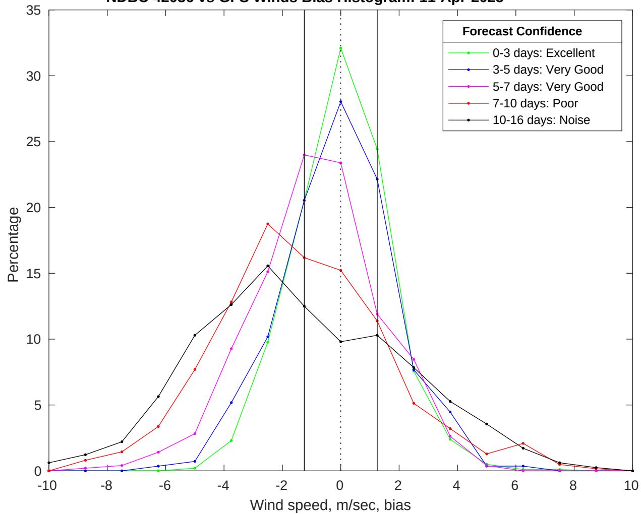
NDBC 42036 vs GFS Winds Bias Histogram: 11-Apr-2025
