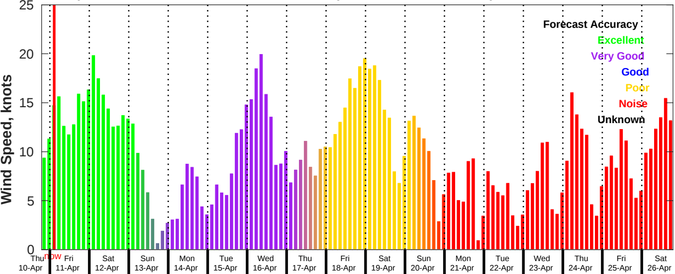
GFS Wind Speed Forecast for NDBC 42036 from 10-Apr-2025 19:00:00 to 26-Apr-2025 19:00:00
