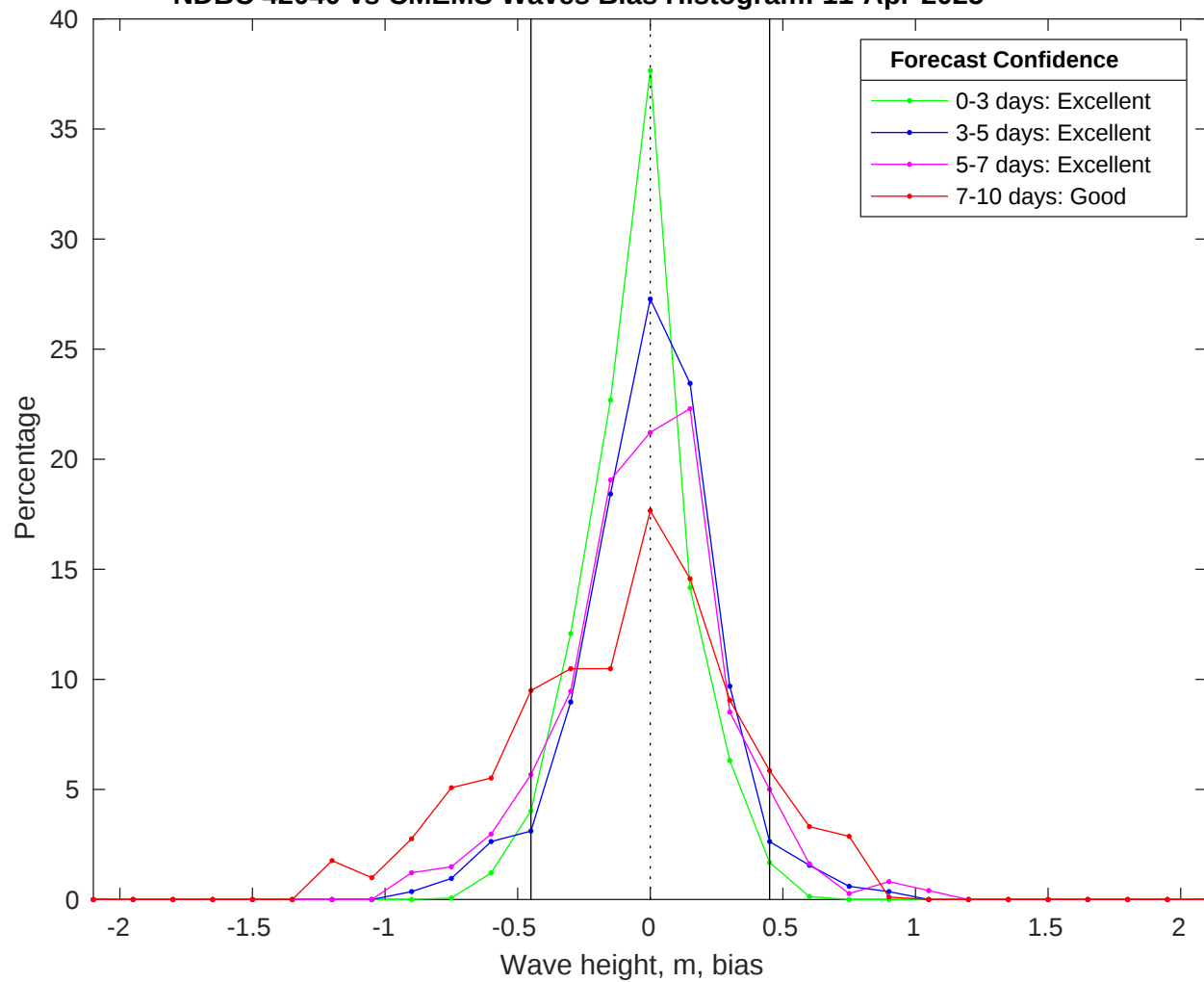
NDBC 42040 vs CMEMS Waves Bias Histogram: 11-Apr-2025
