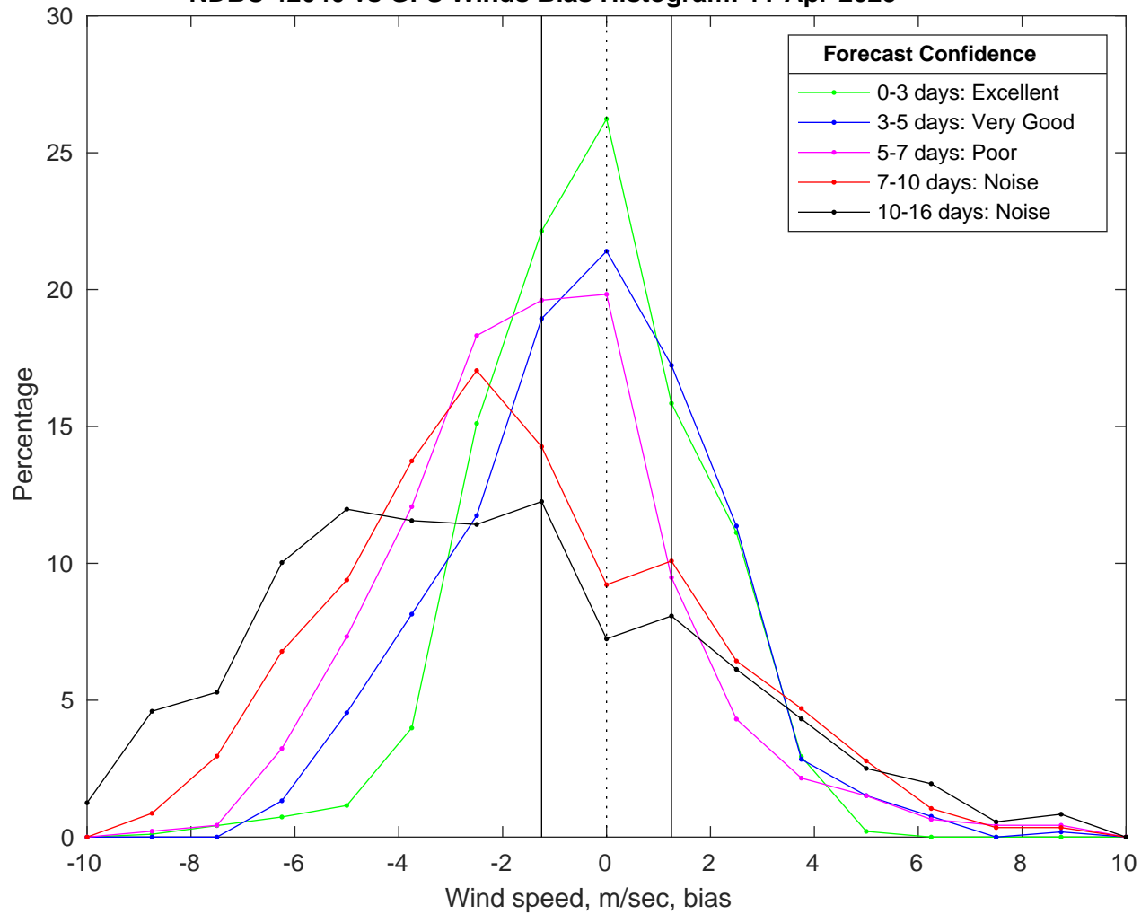
NDBC 42040 vs GFS Winds Bias Histogram: 11-Apr-2025
