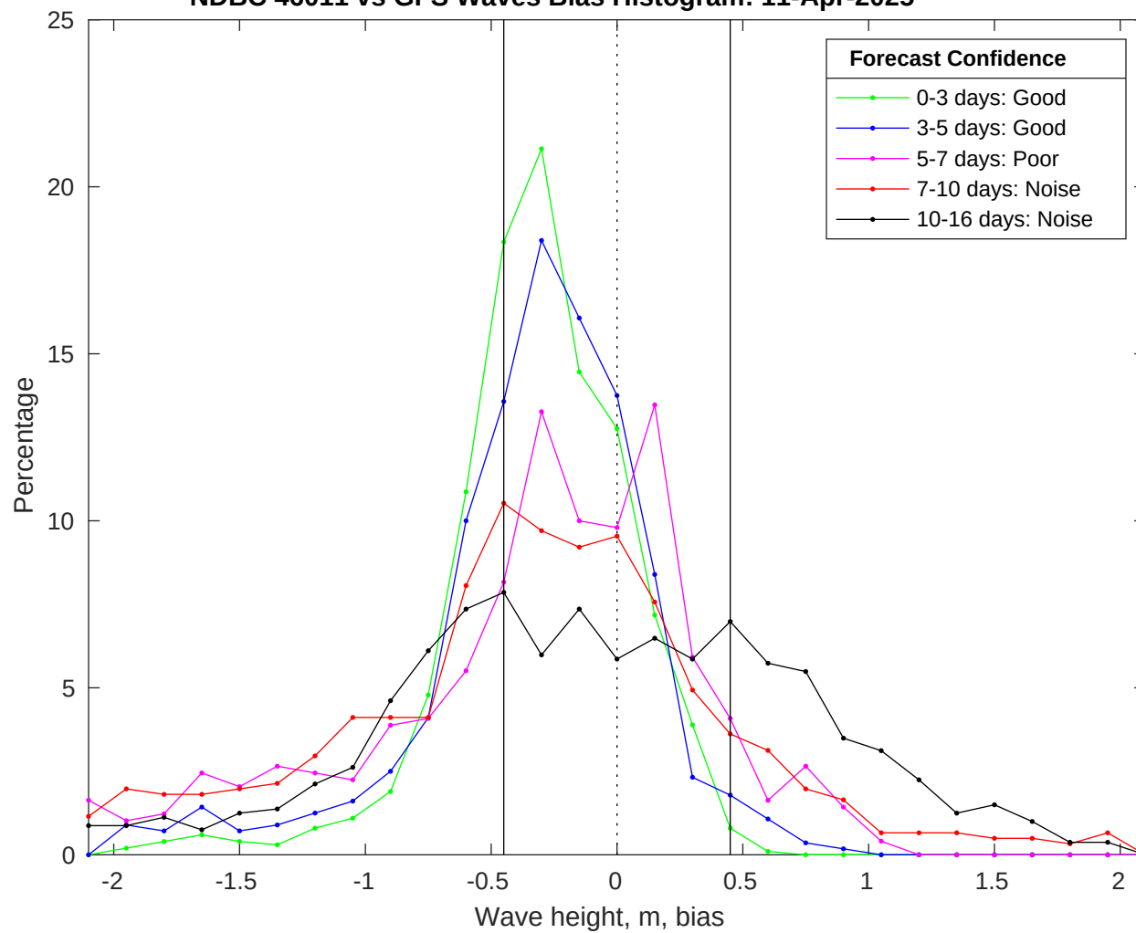
NDBC 46011 vs GFS Waves Bias Histogram: 11-Apr-2025
