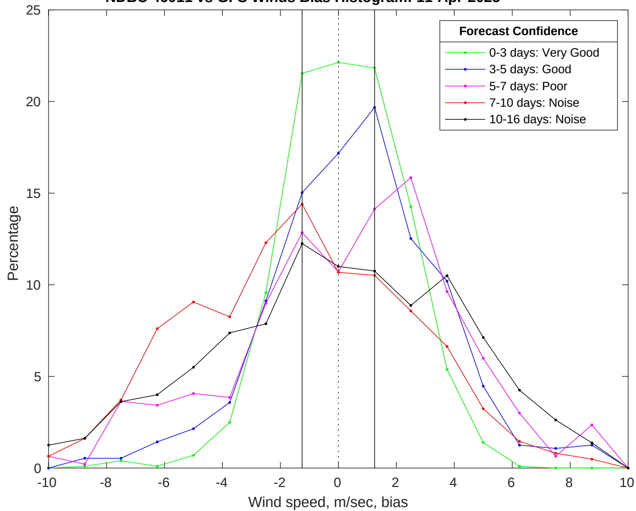
NDBC 46011 vs GFS Winds Bias Histogram: 11-Apr-2025
