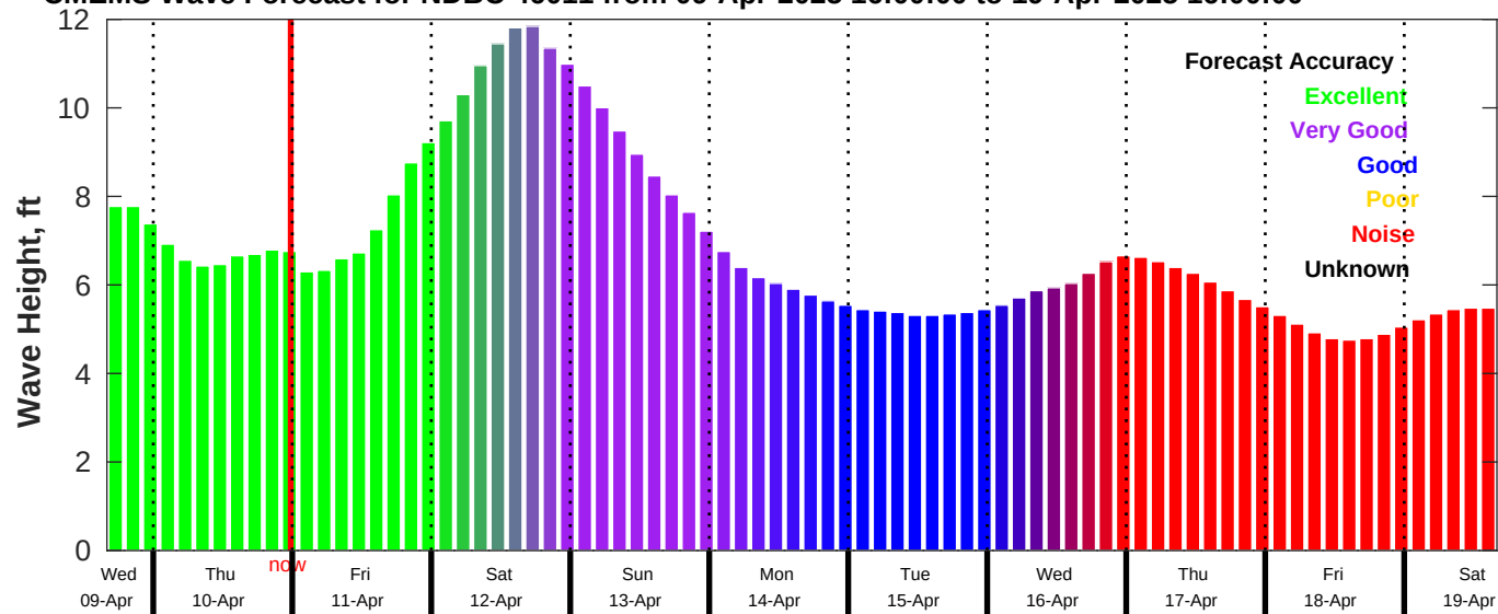
CMEMS Wave Forecast for NDBC 46011 from 09-Apr-2025 16:00:00 to 19-Apr-2025 16:00:00
