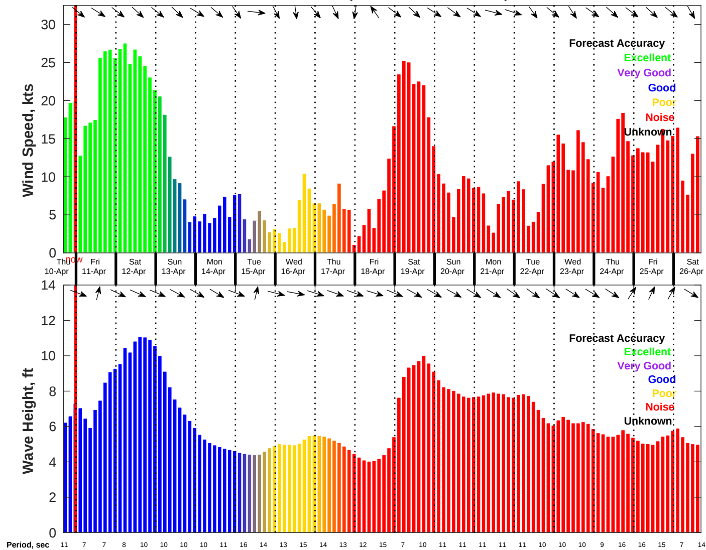
Wind & Wave Forecast for NDBC 46011 from 10-Apr-2025 16:00:00 to 26-Apr-2025 16:00:00
