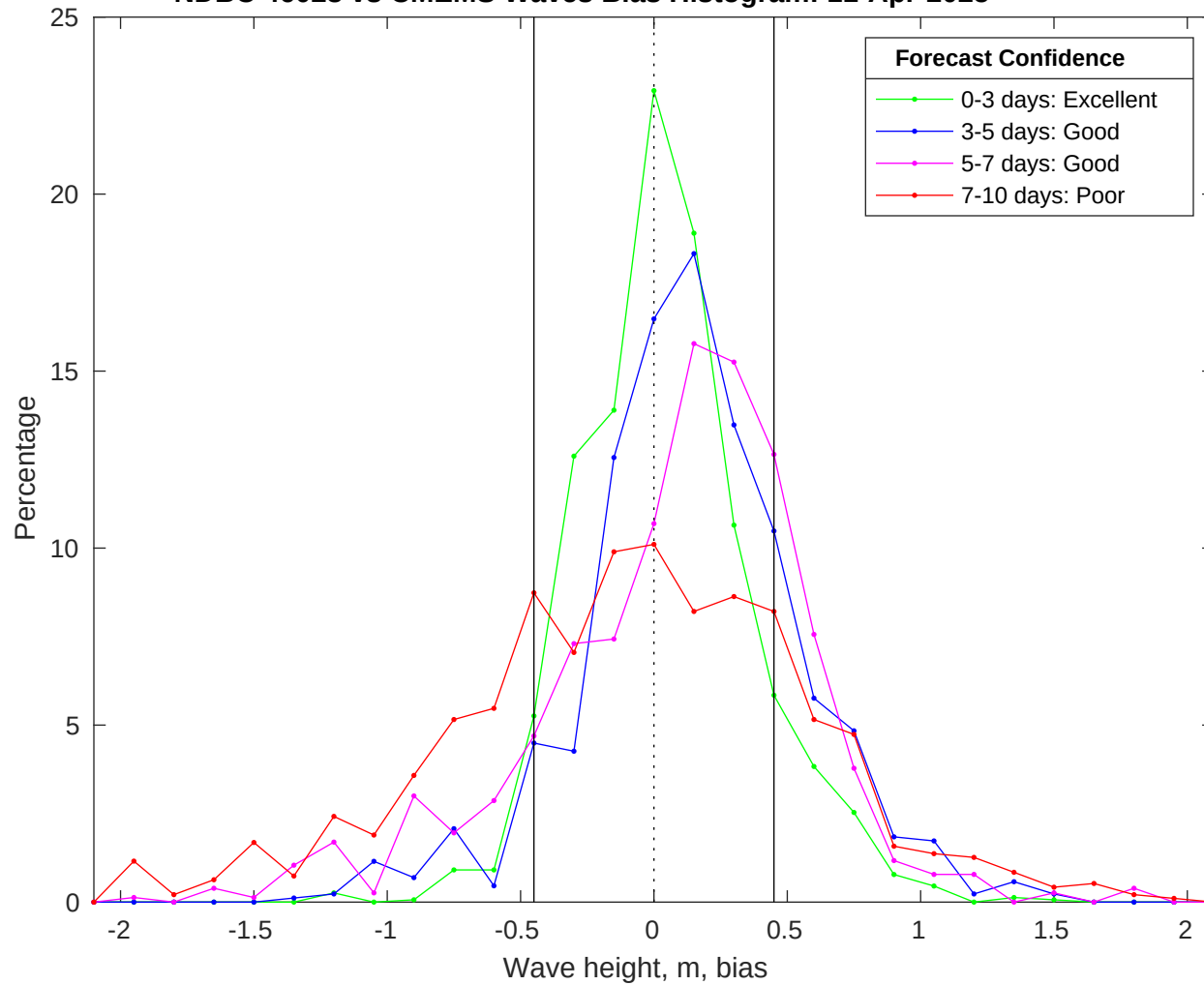
NDBC 46028 vs CMEMS Waves Bias Histogram: 11-Apr-2025
