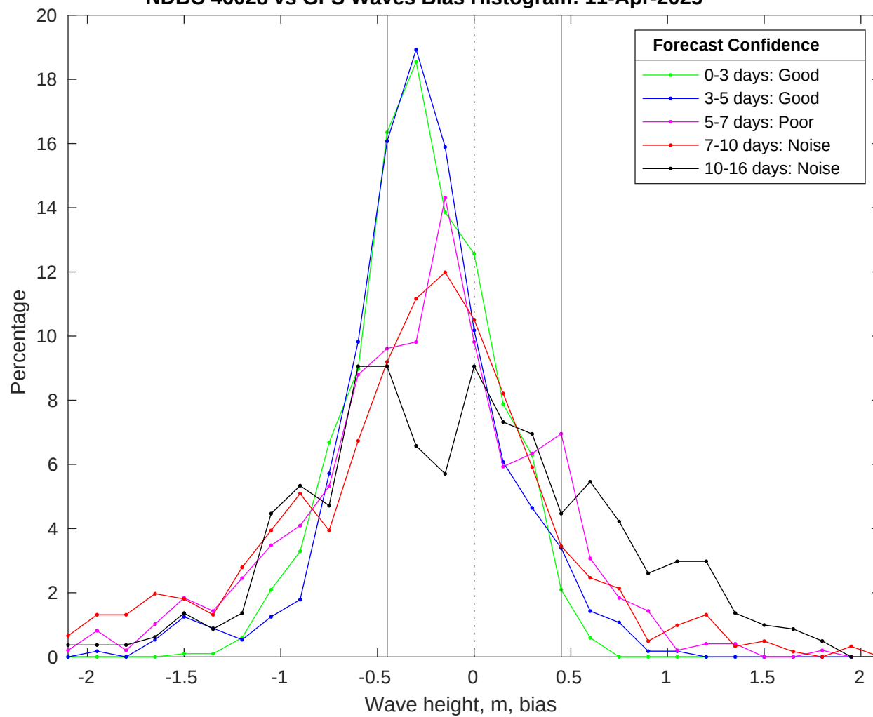
NDBC 46028 vs GFS Waves Bias Histogram: 11-Apr-2025
