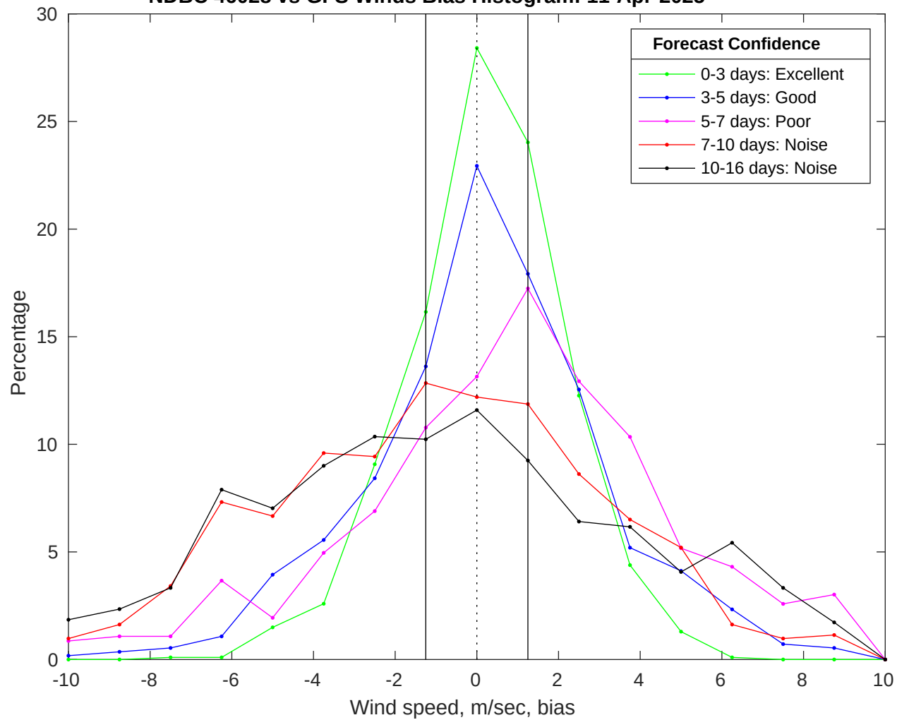
NDBC 46028 vs GFS Winds Bias Histogram: 11-Apr-2025
