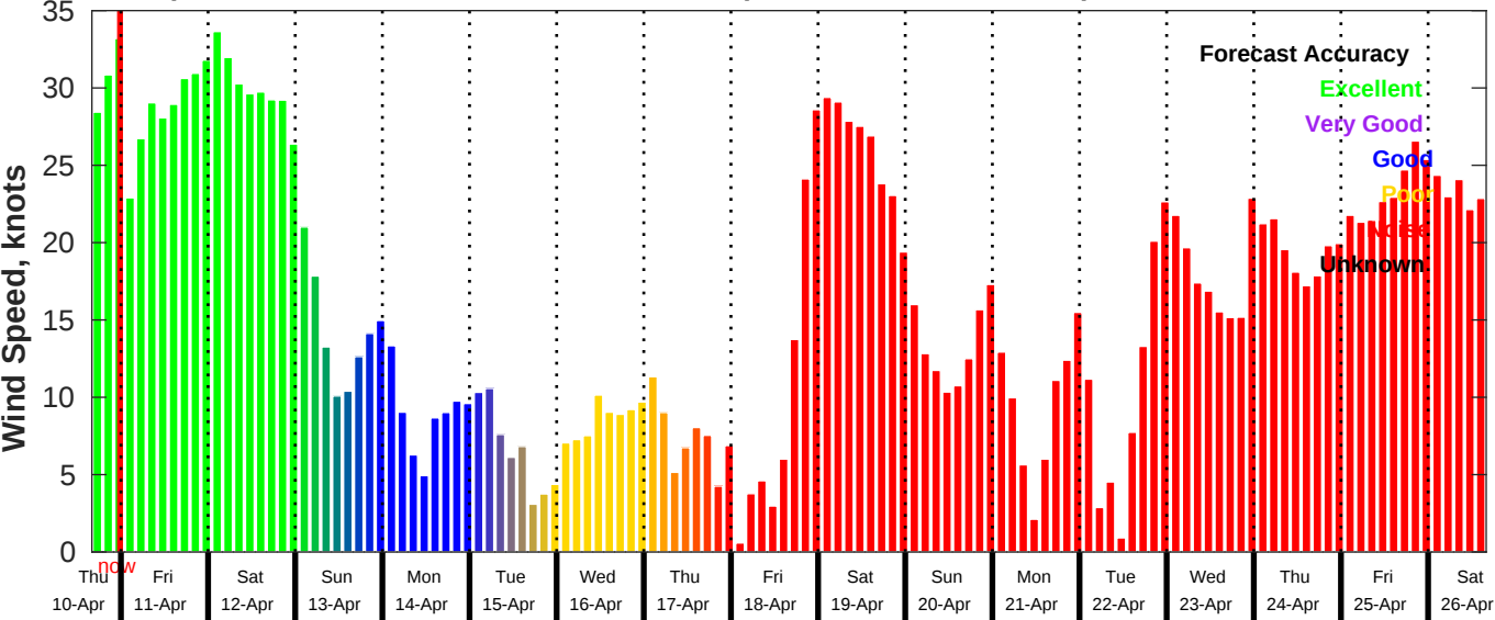
GFS Wind Speed Forecast for NDBC 46028 from 10-Apr-2025 16:00:00 to 26-Apr-2025 16:00:00
