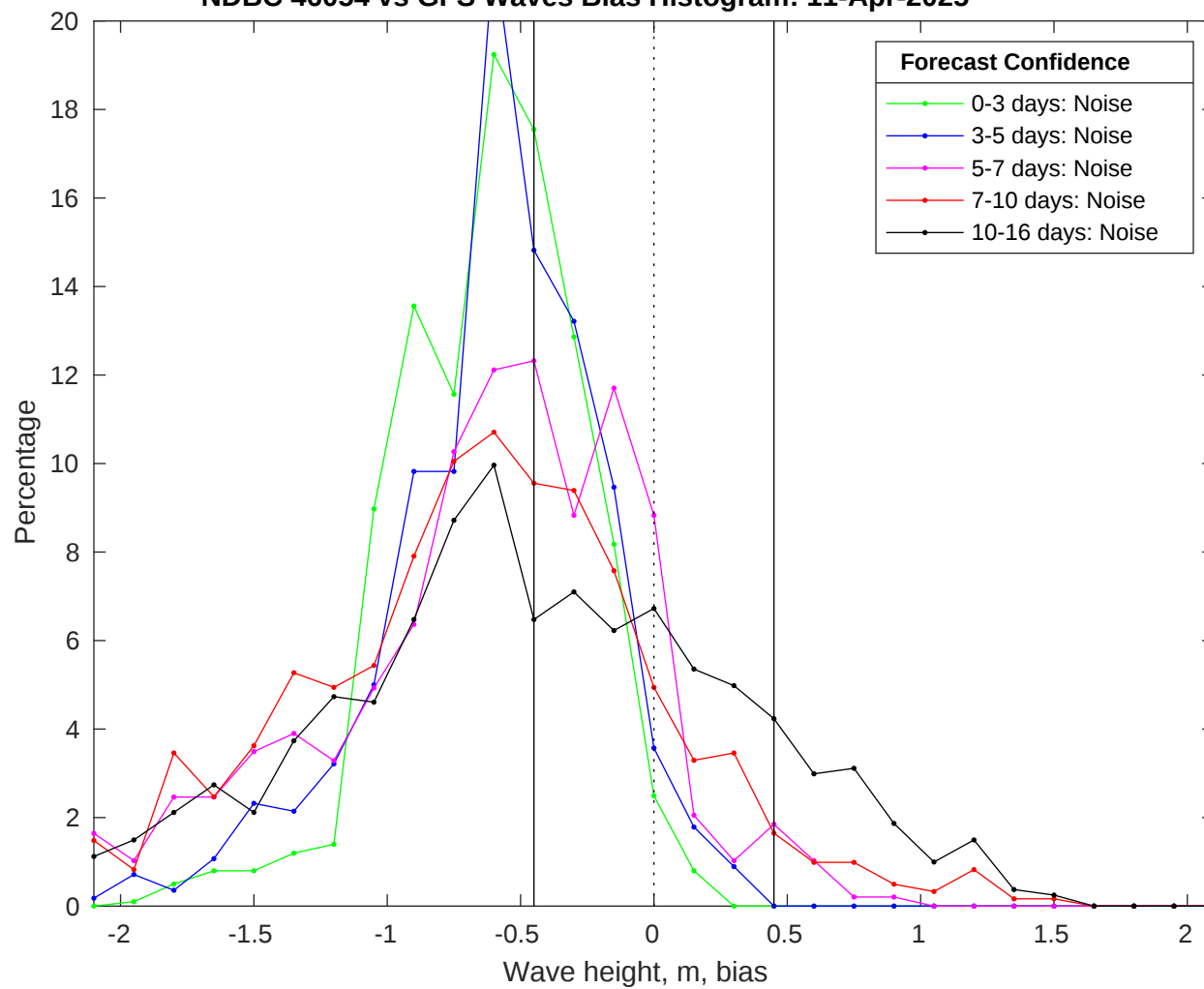
NDBC 46054 vs GFS Waves Bias Histogram: 11-Apr-2025
