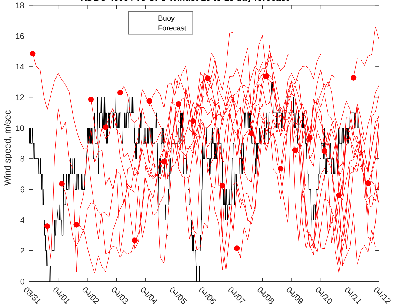
NDBC 46054 vs GFS Winds: 10 to 16 day forecast
