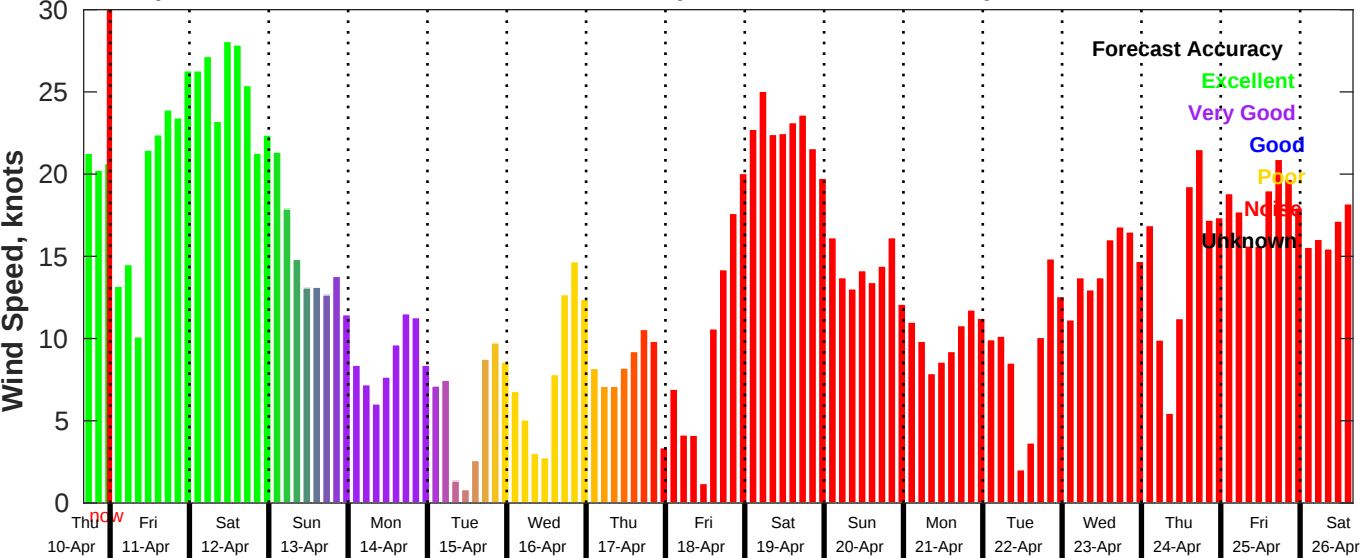
GFS Wind Speed Forecast for NDBC 46054 from 10-Apr-2025 16:00:00 to 26-Apr-2025 16:00:00
