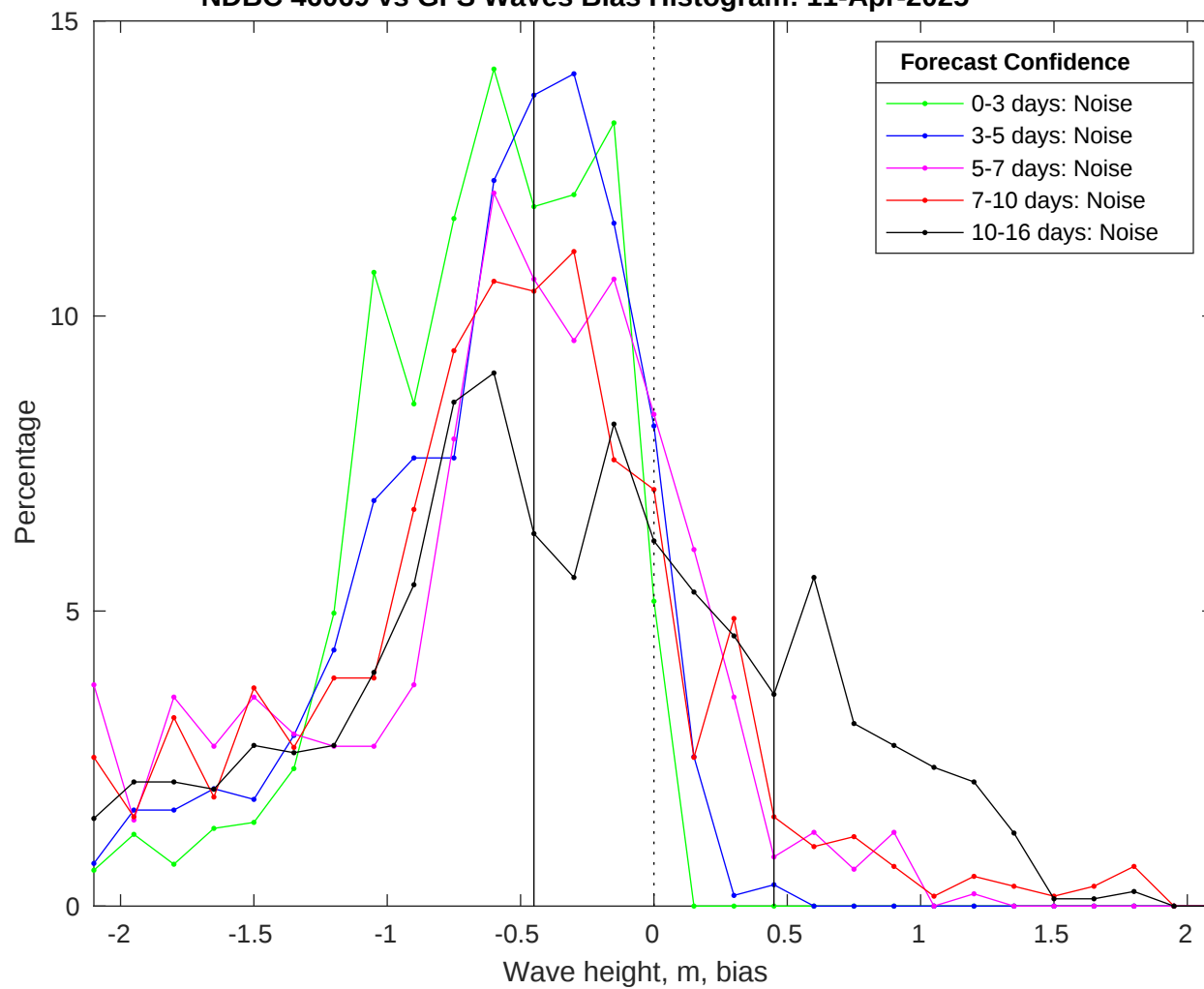
NDBC 46069 vs GFS Waves Bias Histogram: 11-Apr-2025
