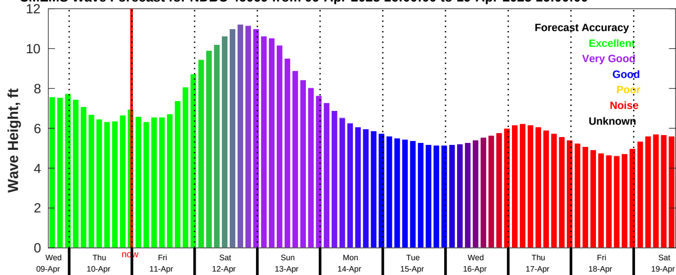
CMEMS Wave Forecast for NDBC 46069 from 09-Apr-2025 16:00:00 to 19-Apr-2025 16:00:00
