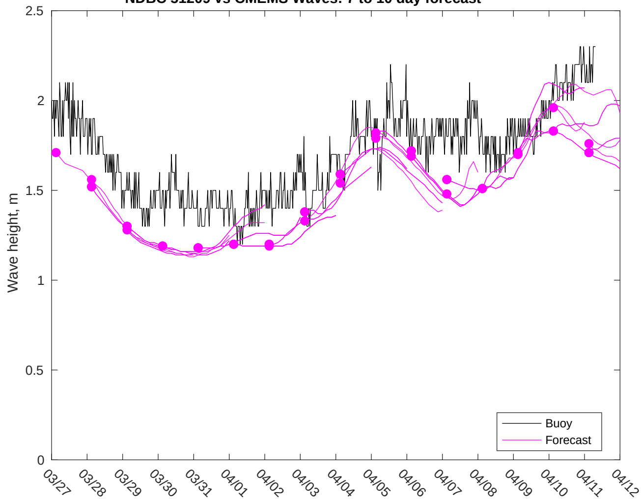
NDBC 51209 vs CMEMS Waves: 7 to 10 day forecast
