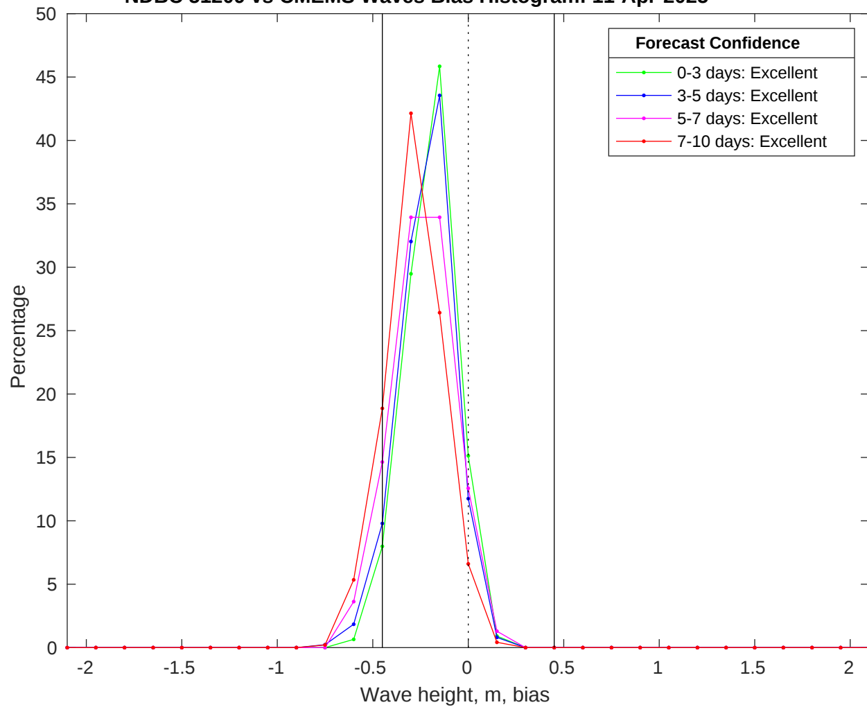
NDBC 51209 vs CMEMS Waves Bias Histogram: 11-Apr-2025
