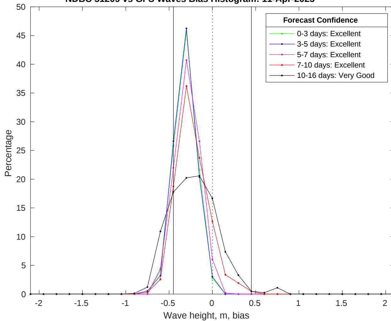
NDBC 51209 vs GFS Waves Bias Histogram: 11-Apr-2025
